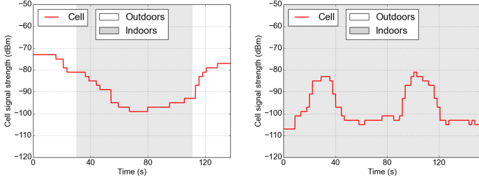
(a) Cell signal at transition (b) Cell signal variations in indoor Figure 4. (a) At a transition, cell signal can change by less than 15dBm in 10 seconds. (b) During movements inside a building, cell signals can change faster than 15dBm in 10 seconds.
